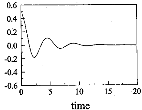
FIGURE 3: Simulation Result of 1 DOF System !! ! (k_p, k_d) = (2, 0.3)
