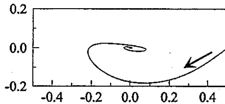
FIGURE 6: Simulation Result of 2 DOF System !! ! (k_p, k_d) = (1, 0.3)
