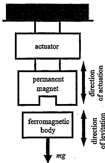
FIGURE 1: Outline of Magnetic Suspension System
