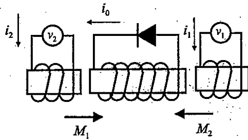
FIGURE 1: Outline of rotor with rectified circuit coil
