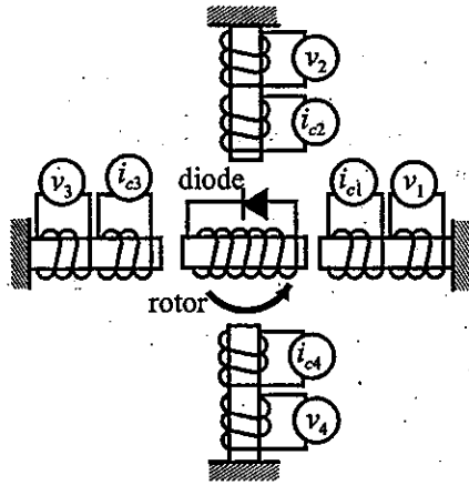
FIGURE 3: Schematic illustration of bearingless motor I (radially excited rotor type)
