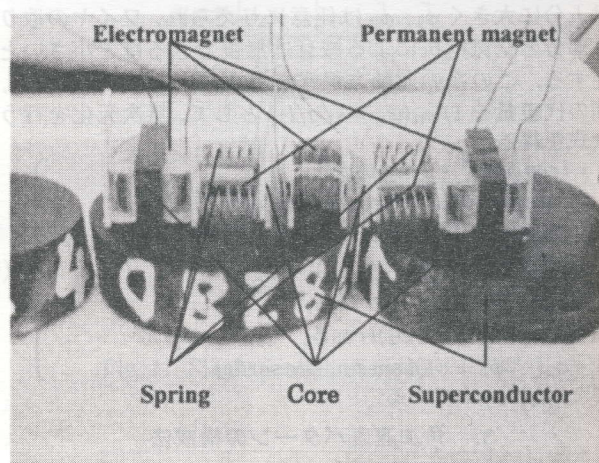
Fig. 2 Experimental device
