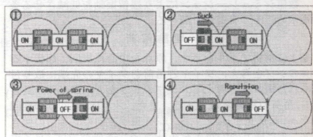
Fig. 1 Movement principle
