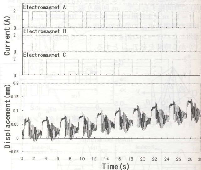
Fig. 3 Experiment result
