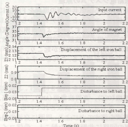
Fig.3 Step response to the left iron ball
